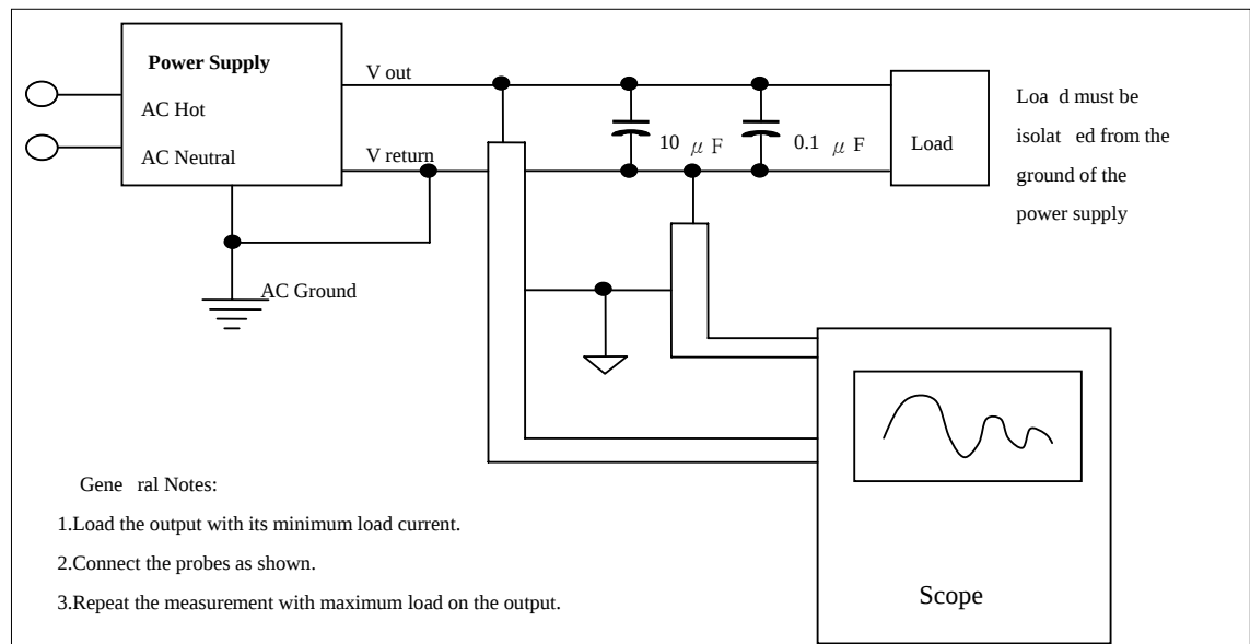
Figure1. Differential Noise Test Setup
